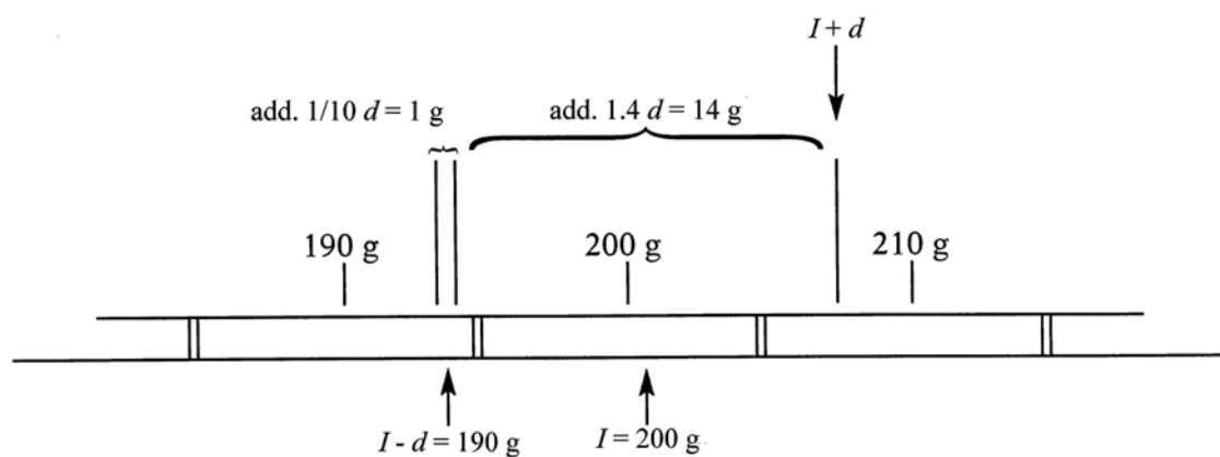
Figure 10 – Instrument with d = 10 g
